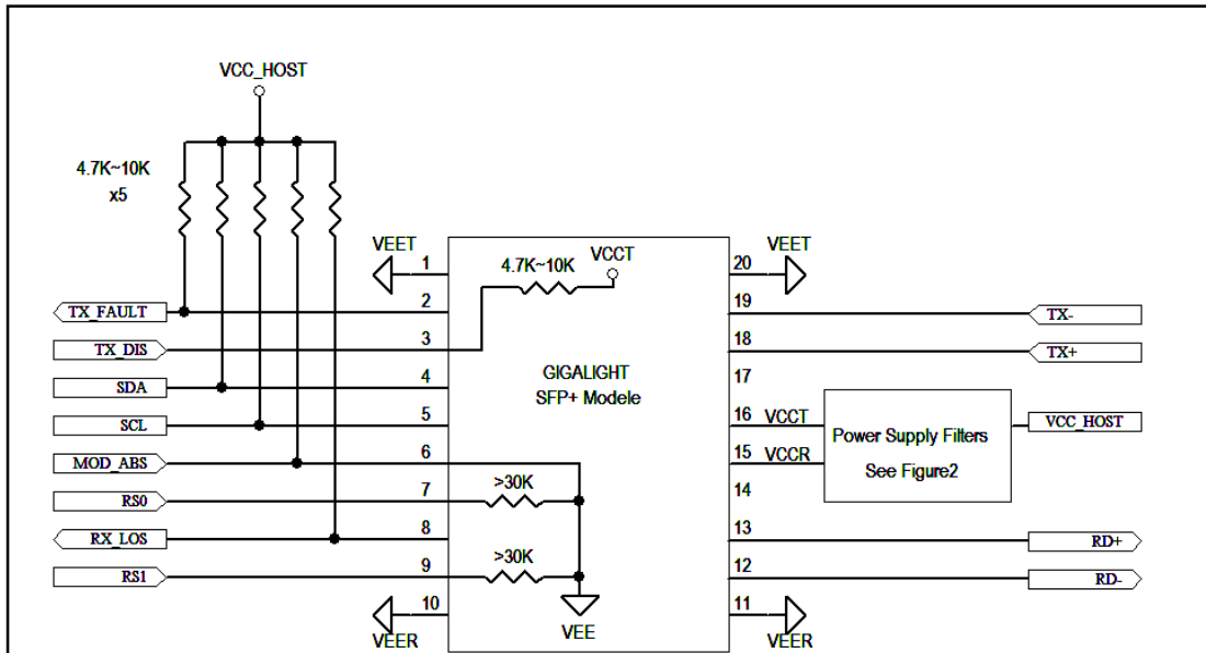
Figure3. Host-Module Interface
