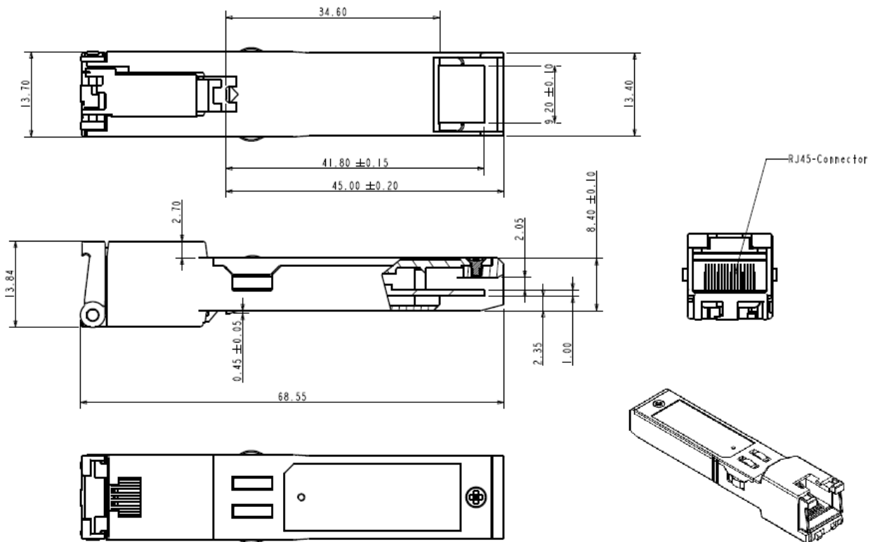
Figure 2. EE-FB-PxRC mechanical dimensions
