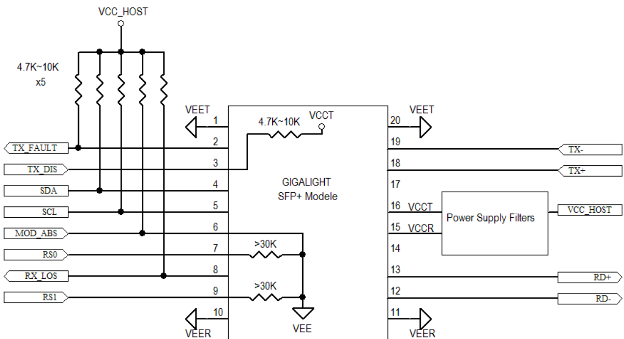
Figure5. Host-Module Interface
