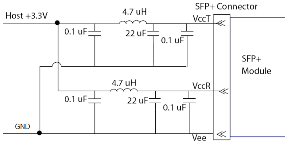
Figure4. Host Board Power Supply Filters Circuit
