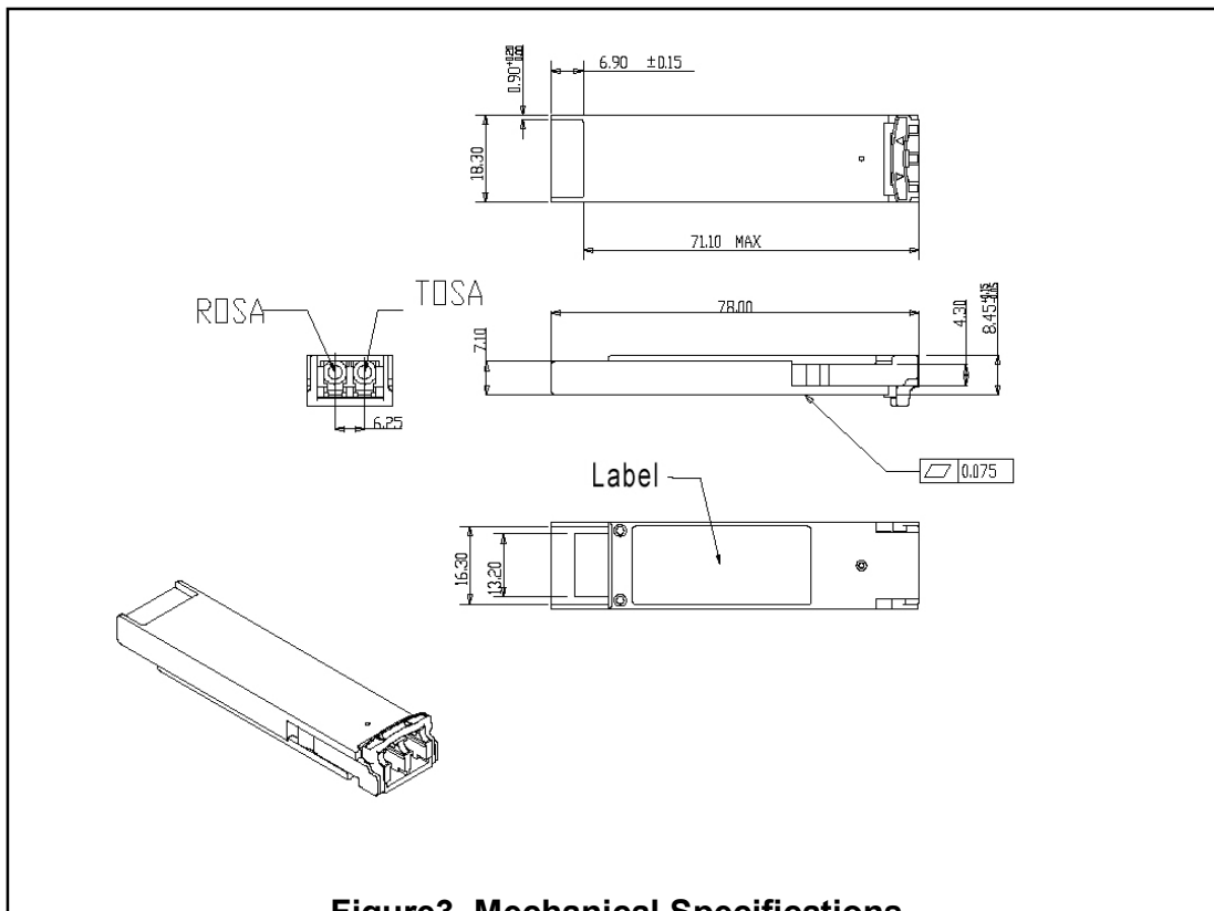
Figure3. Mechanical Specifications
